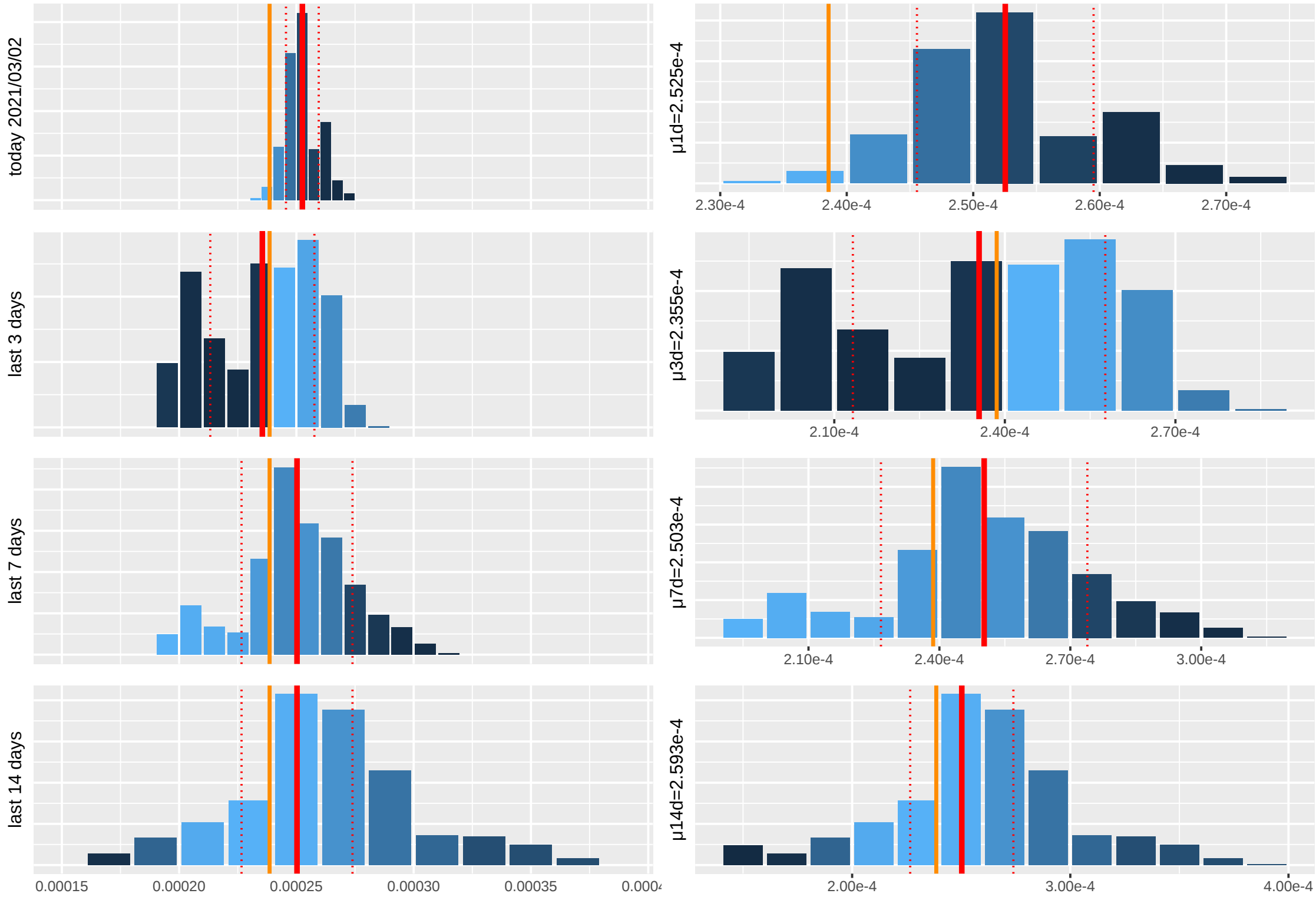
CryptoMarketPlot.com: histograms of Pancakeswap price distribution, orange: \mu_{1h} , red: \mu \pm 1 \cdot \sigma , darker=older
