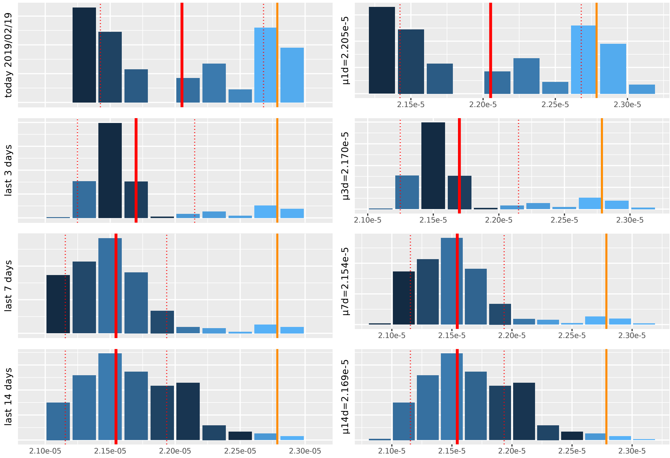
CryptoMarketPlot.com: histograms of Stellar price distribution, orange: \mu_{1h} , red: \mu_{t \pm 1 * \sigma_t} , darker=older
